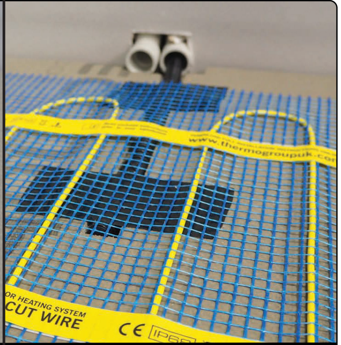
Ensure the floor sensor conduit is located evenly between two runs of heating cable.
